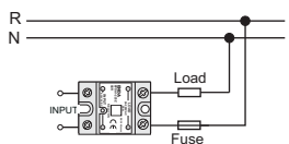
Single Phase Load Application
