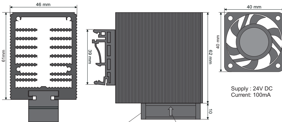
ETS-46-62 HEATSINK
